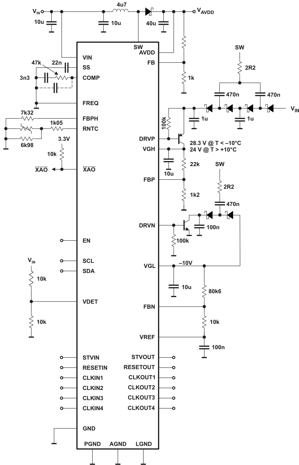
Figure 40. Typical Application Circuit Using Positive Charge Pump in \times 2.5 Configuration
